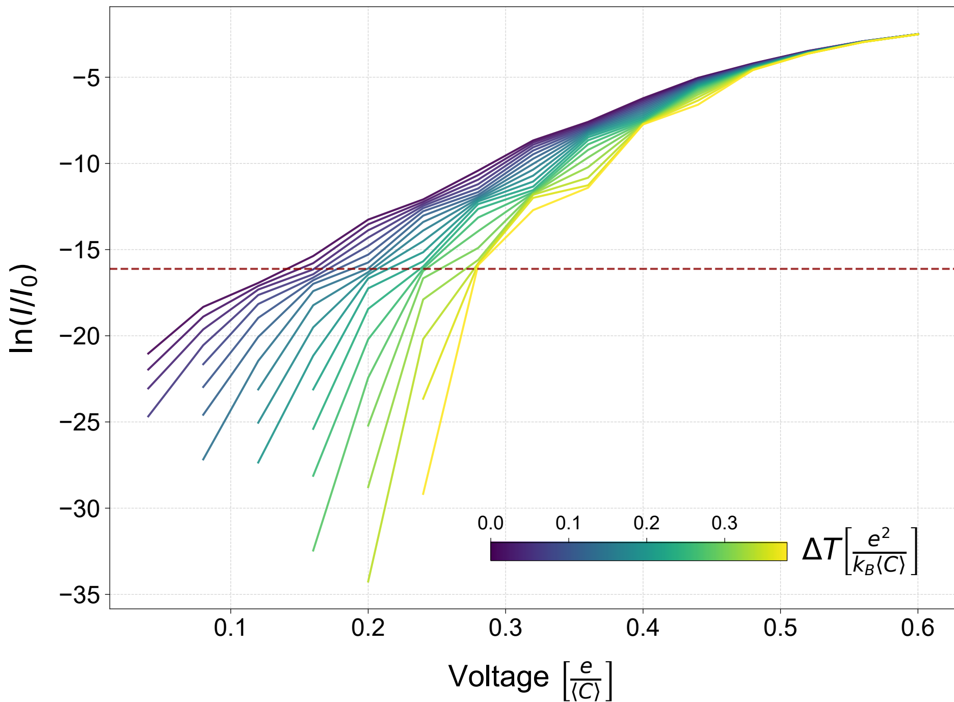
Semi-Log I-V for Fixed Island Temperature T = 0.4E_c
